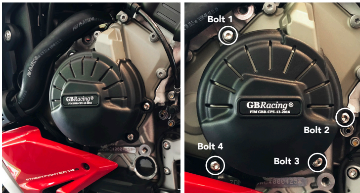
Bolt 4 M6X35A2-TORX - 10Nm
