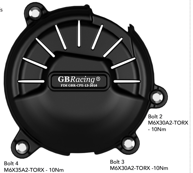
Bolt 1 M6X30A2-TORX - 10Nm
